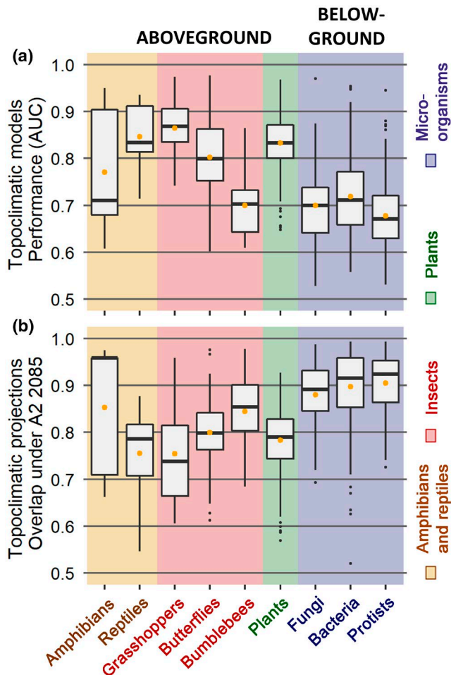
FIGURE 1 The role of topoclimate and climate change in defining current and future taxa distributions. (a) Performance as measured with AUC per taxon of the topoclimate ensemble models. The model performance of above-ground species is significantly better than the model performance of below-ground microorganisms ( p < .001 ; measured with Wilcoxon rank sum test). For other evaluation metrics and per technique (Generalized Linear Model, Generalized Boosting Model, Artificial Neural Network, Classification Tree Analysis), and for plant genera and soil microorganism orders, see Figure S26 in Appendix S2. (b) Spatial overlap in predicted probability of occurrence (PPO) between current and future (A2 2085 scenario) projections within the whole study area. For other scenarios, plant genera, soil microorganism orders and environmentally analogous areas, see Figure S28 in Appendix S2. Boxes in boxplots span the 25th–75th quartile, with median (black bar) and mean (orange point) in the middle. Whiskers span the lowest and highest scores, yet in maximum to 1.5 \times (75\text{th} - 25\text{th quartile}) ; outlier scores are indicated by black dots
