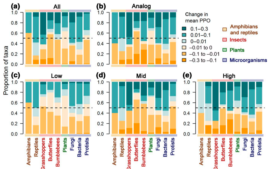
FIGURE 3 Proportions of taxa with different mean changes in predicted probability of occurrence (PPO; classified to six classes) under A2 scenario for 2085. (a) Across the total study area. (b) Across an environmentally analogous part of the study area. (c–e) At different elevational bands (low = <1,180 m a.s.l.; mid = 1,180–1,650 m a.s.l.; high > 1,650 m a.s.l.). For other scenarios and taxonomic ranks, see Figures S43 and S46 in Appendix S2. For median changes, see Figures S47–S49 in Appendix S3
